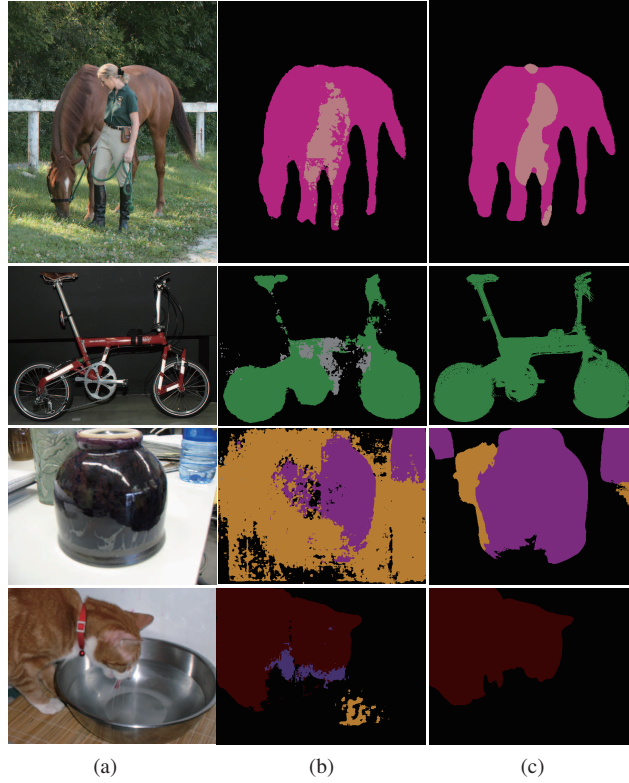
Figure 4 (Color online) Obvious false recognitions are evident in column (b), which can be corrected by using a CRF model. The post-processed results obtained using the CRF approach are shown in column (c).
